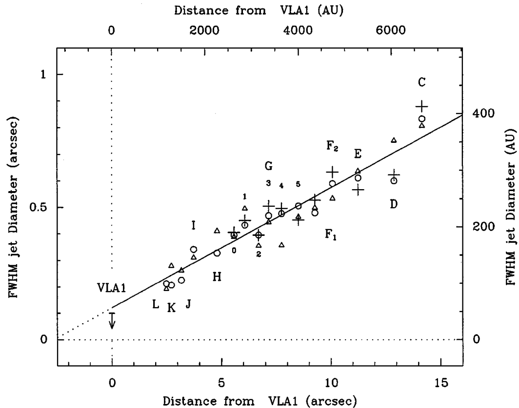
Figure 9 The deconvolved FWHM jet diameter along the HH 1 jet as a function of distance from the driving source. Based on images of [FeII] ( circles ), H 2 ( triangles ), and [SII] ( pluses ) from the Hubble Space Telescope. [From Reipurth et al. (2000a).]
