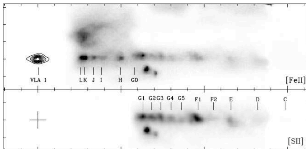
Figure 8 The tiny radio continuum jet around the HH 1 source is seen together with infrared [FeII] and optical [SII] images of the HH 1 jet from the Hubble Space Telescope.
